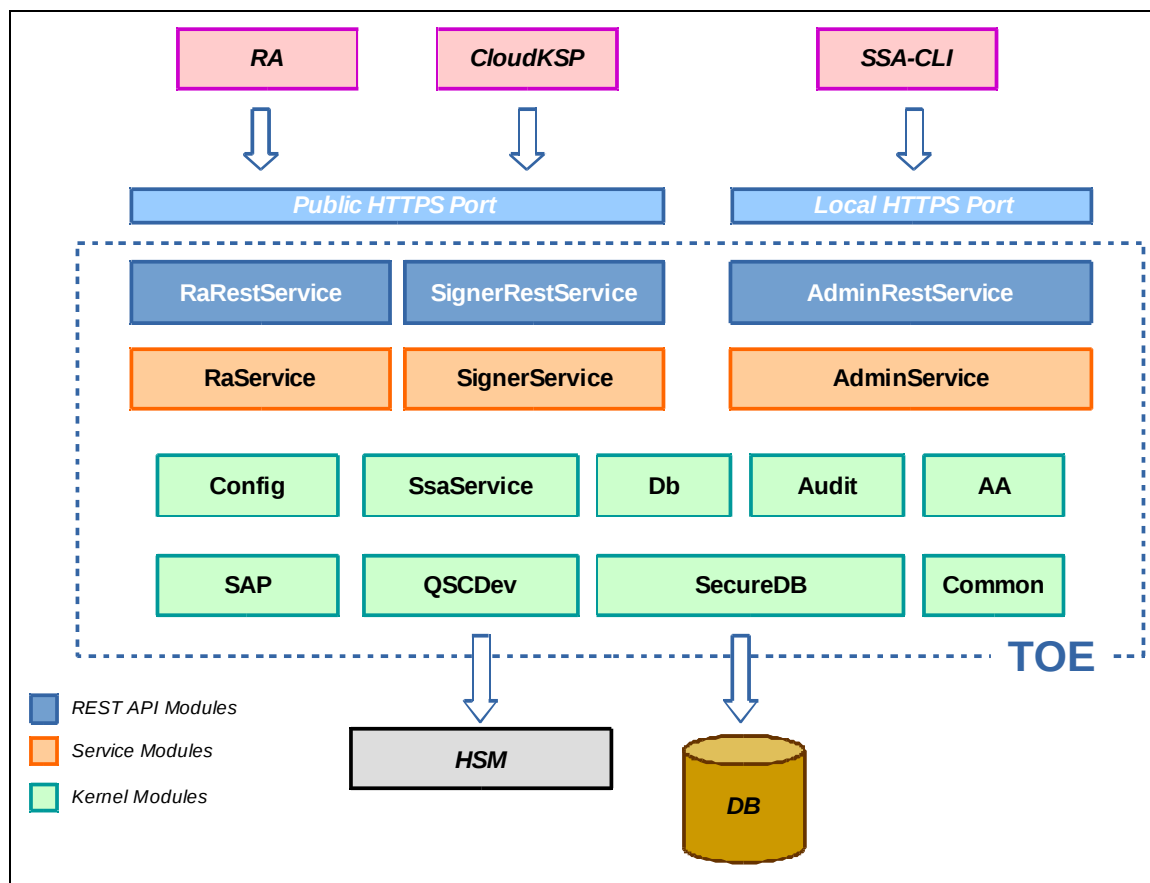
Figure 2 - TOE logical architecture
