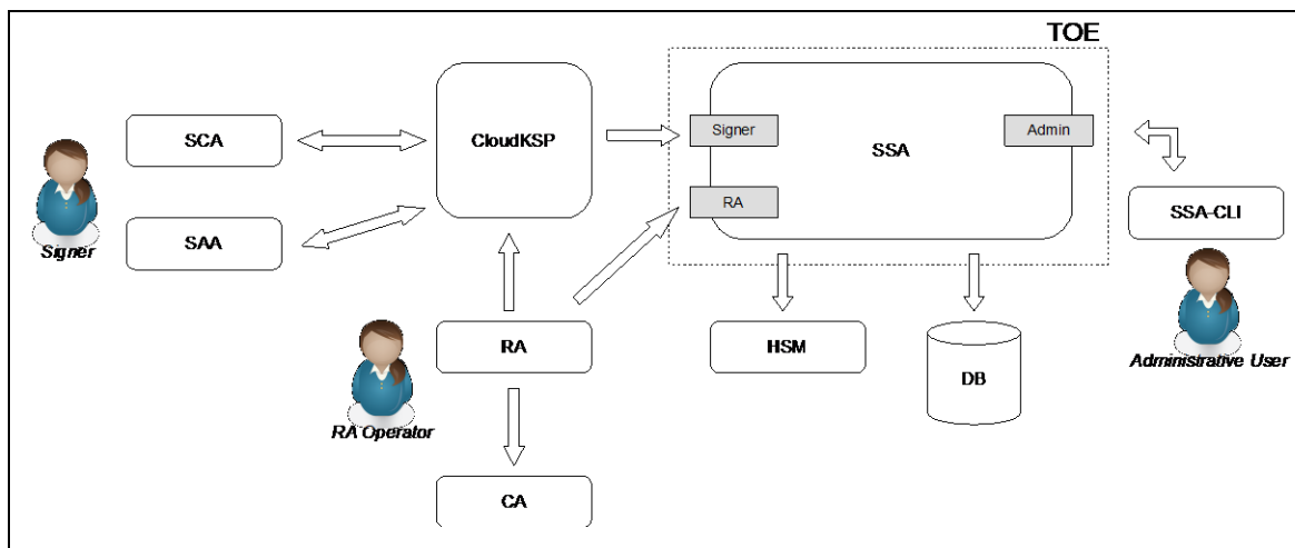
Figure 1 - TW4S solution including the SSA (TOE) with its interfaces and users
