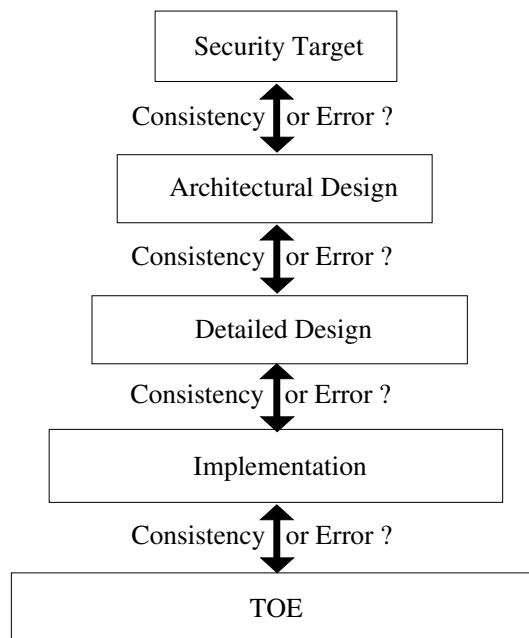
Figure 3.3.1 Representations of the TOE and Correctness
