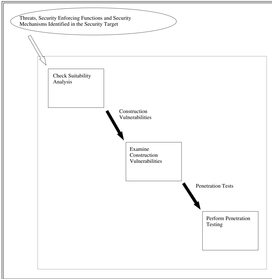
Figure 4.4.3 Example Activity Dependencies
