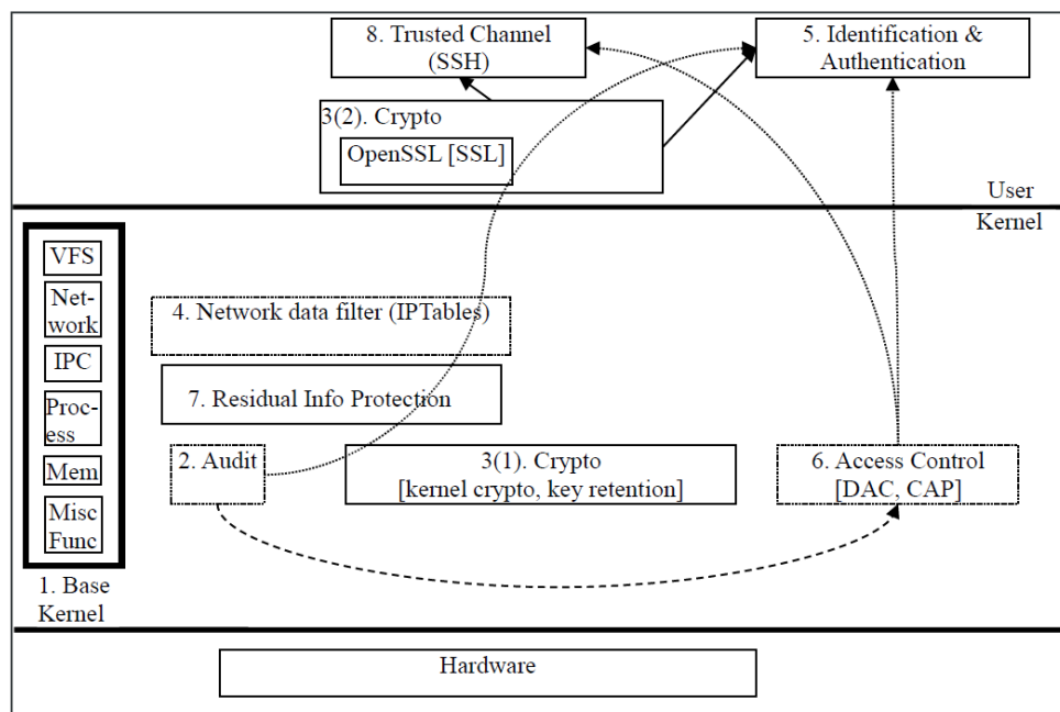
Figure 1. TOE subsystems and interactions among them
