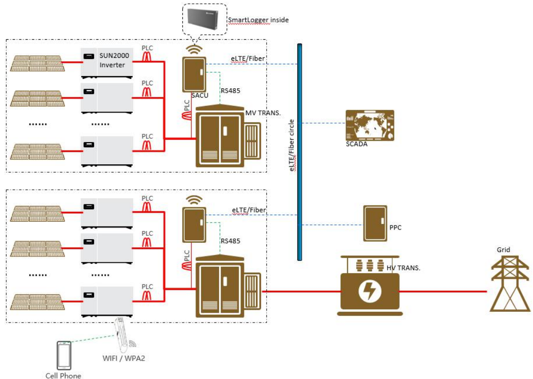
Figure 1-1 Position of the SUN2000HA inverter on the entire PV plant communication network
