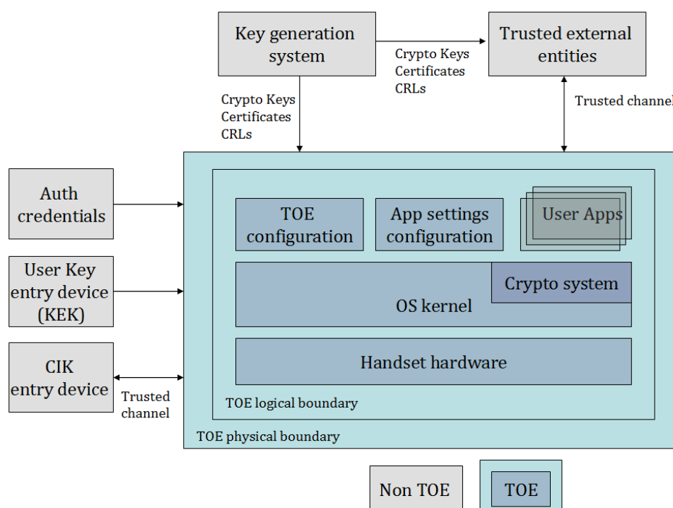
Figure 1: TOE boundary
