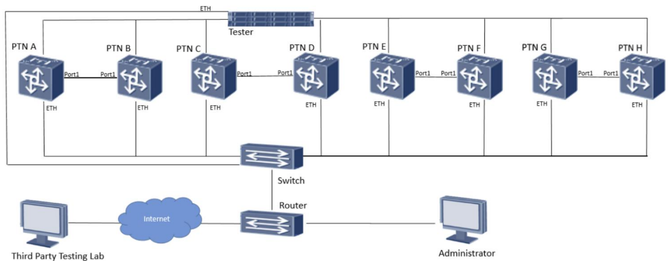
Figure 1-2 TOE Deployment Diagram
